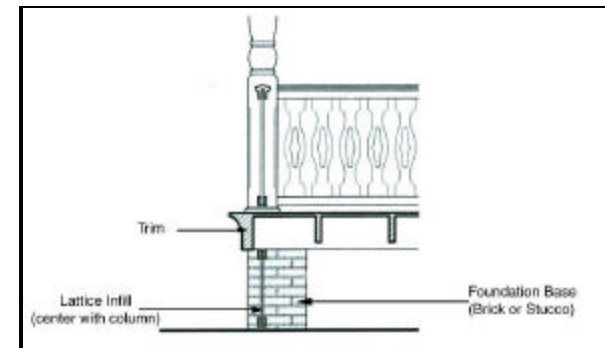
Foundation Detail
